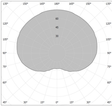
cd/klm C0 - C180 ..... C90 - C270 Photometry (polar plot) \eta = 78\%
